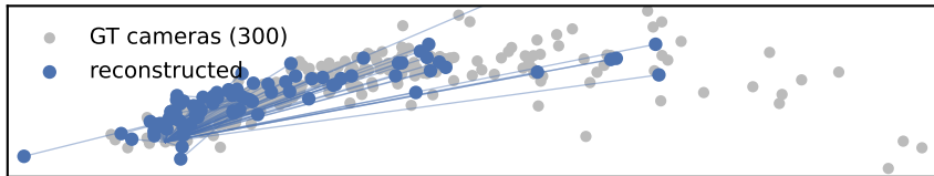
SS-RESfM (MAD, label-free) registered 67/300, translation median 3.8, mean 9.9
